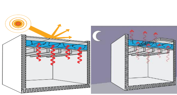
Fig. 14: Roof Pond performance. Source: Roche, 2024
